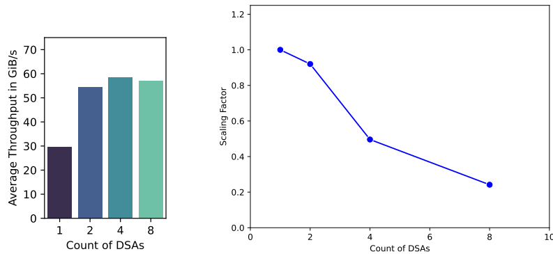
(a) Average Throughput for different amounts of participating DSA.
