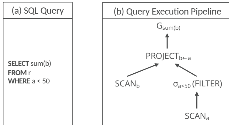
Figure 6.1: Illustration of the benchmarked simple query in (a) and the corresponding pipeline in (b). Taken from [2, Fig. 1].
